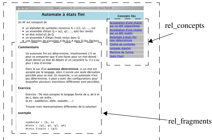
Fig. 6. Instance of a composite node
