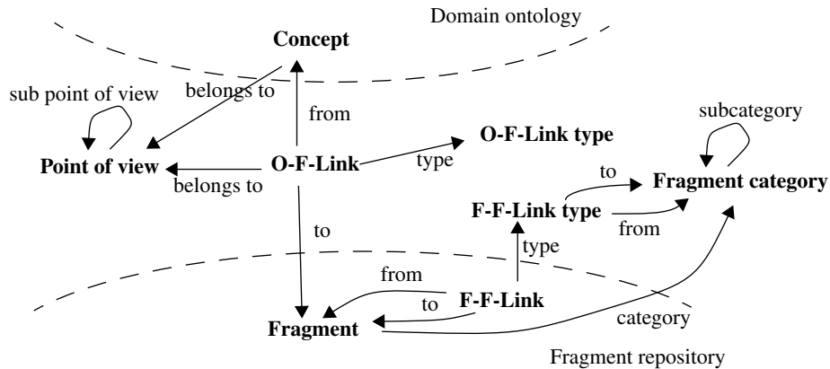
Fig. 3. Classes of the hyperbook ontology
