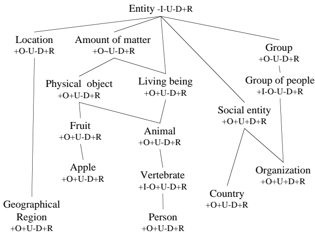
Figure 4: Restricting to rigid properties.
