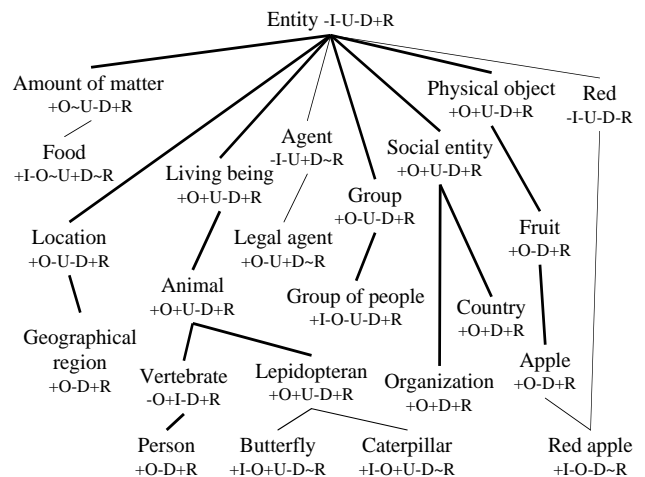
Figure 6: The final taxonomy with highlighted backbone.
